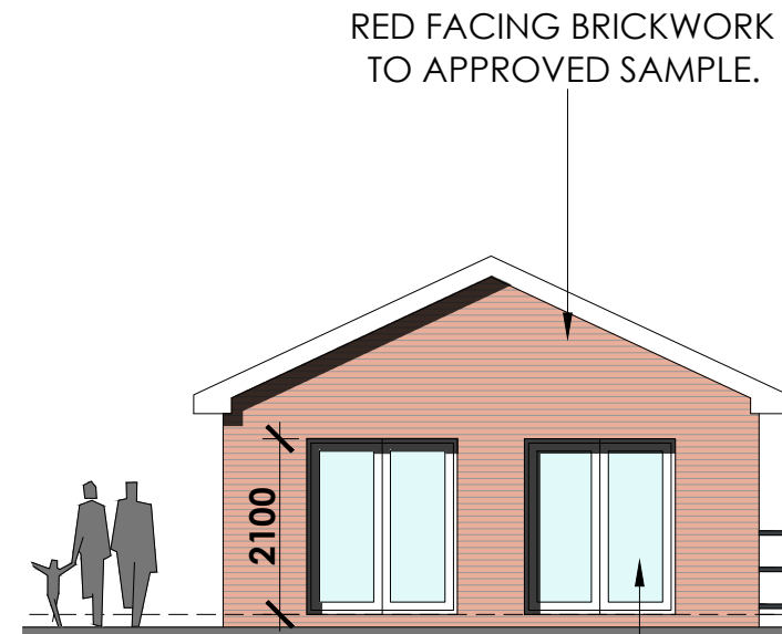
FRONT ELEVATION
