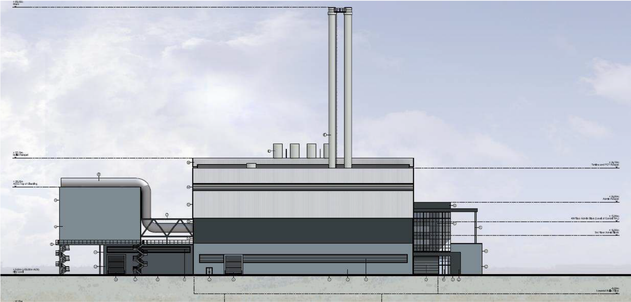
Figure 1.7: Main ERF Building north elevation
